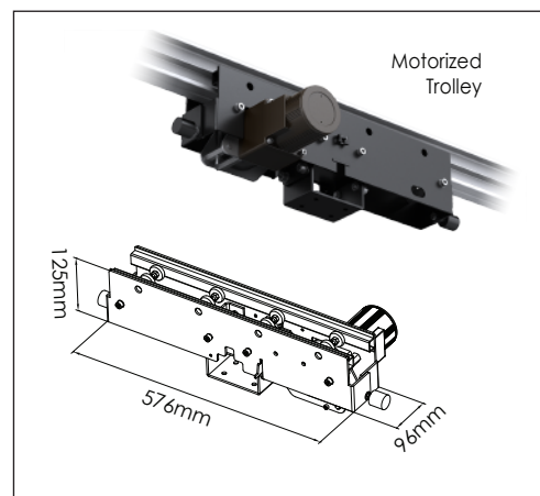
Motorized Trolley can be hung on & Travelled with Top Rail
